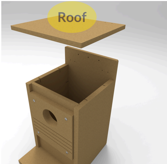
Attach part roof with hinges
