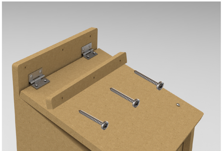
Attach Water Guard to Fence With Longer Screws
