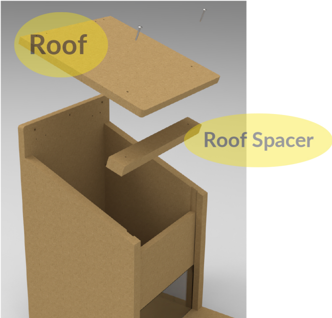
Attach Roof Spacer to Roof With Shorter Screws
