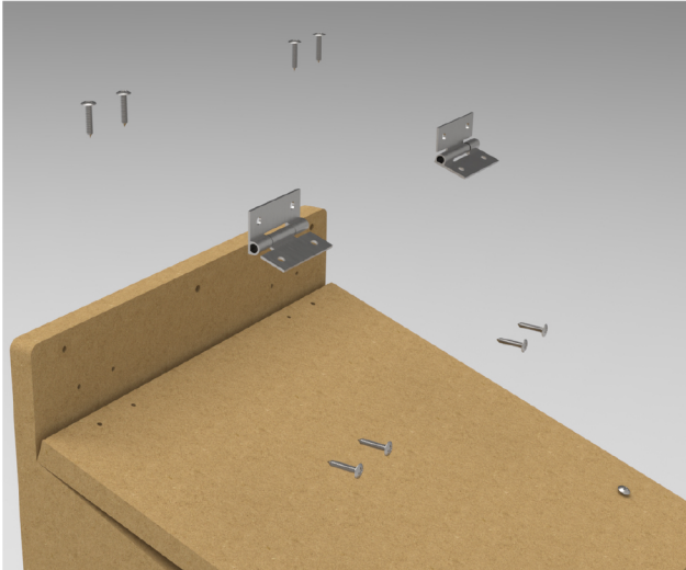
Attach the hinges
